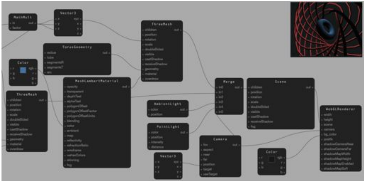
Figure 8: ThreeNodes.js
